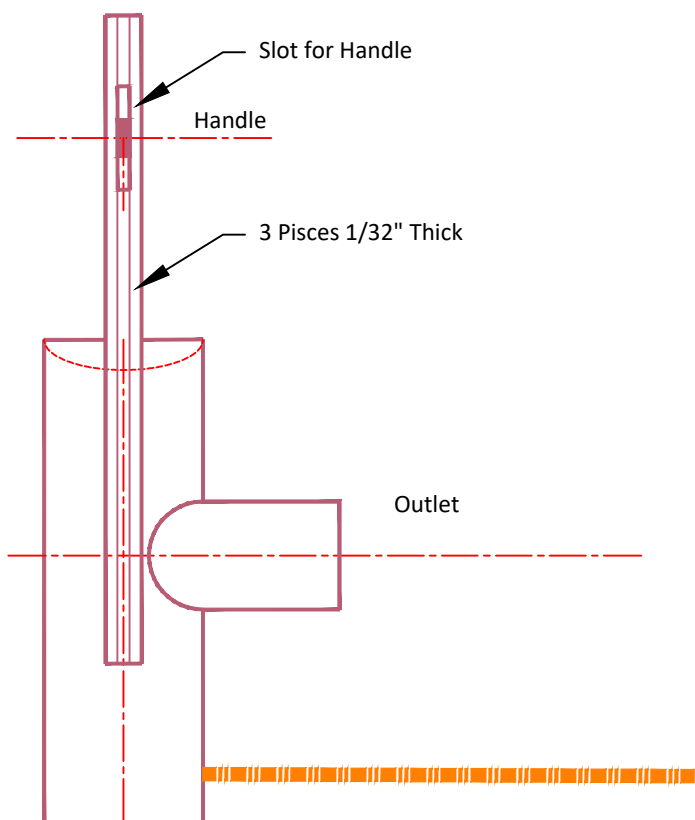
Handel Support Detail Not to Scale
