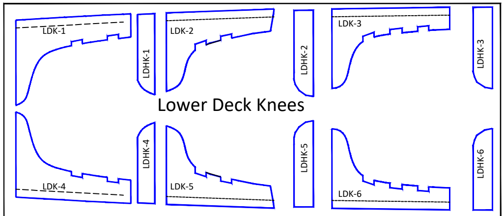
Lower Deck Framing Patterns
