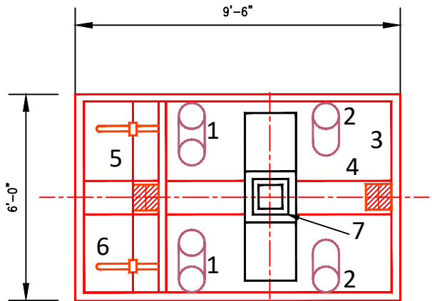
Well Plan
