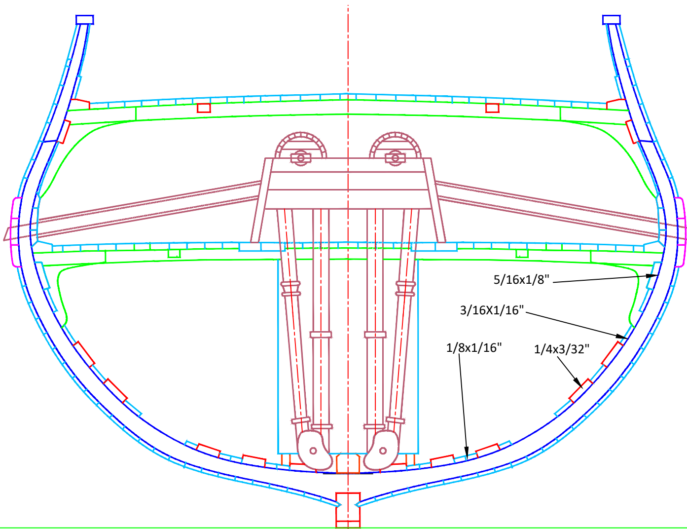
Chain Pumps Pump Details 1:48 sht 2
