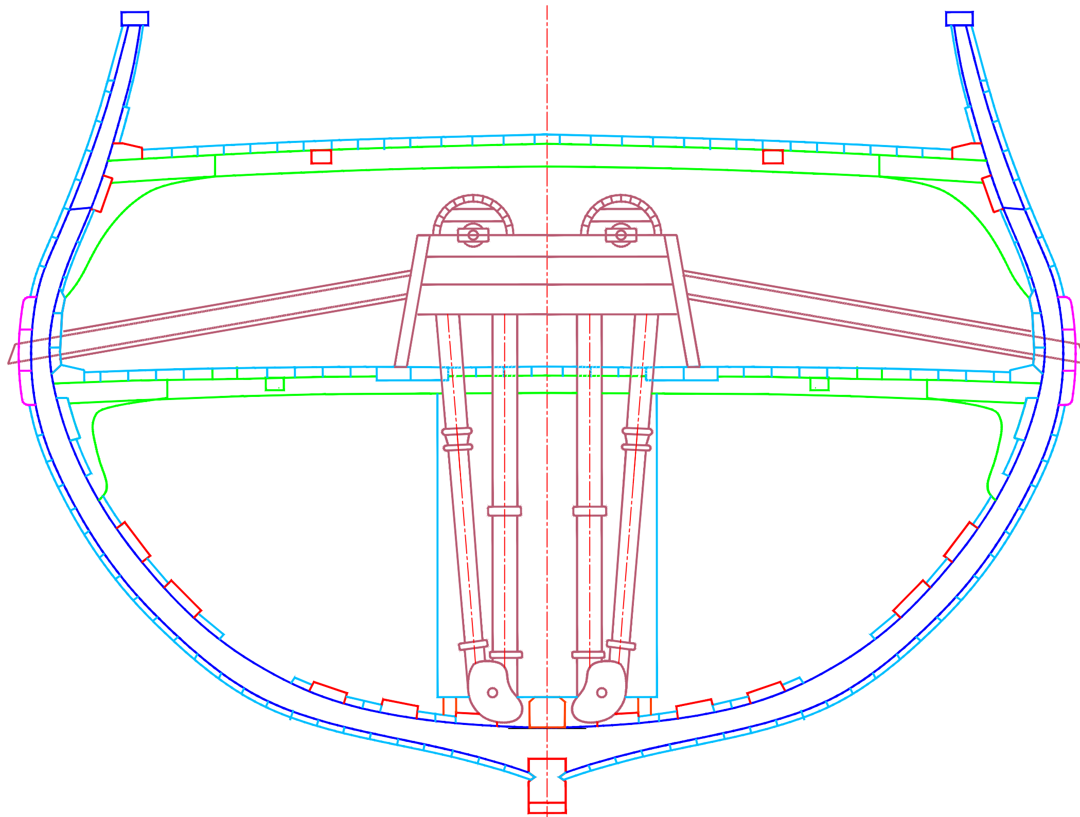
Chain Pumps End View Pump Details 1:32 sht 2
