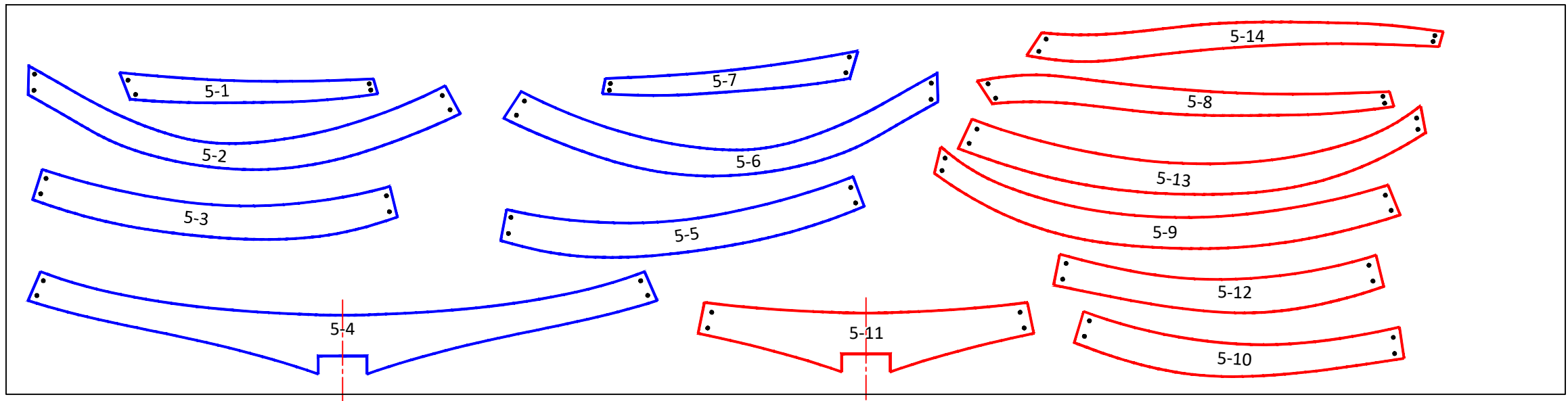
Patterns 1 - 7 for Frame 5 Forward
